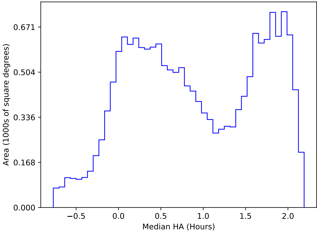
internal_u_expt27_nscale1.1v3.4_10yrs WFD r band: Median HA
