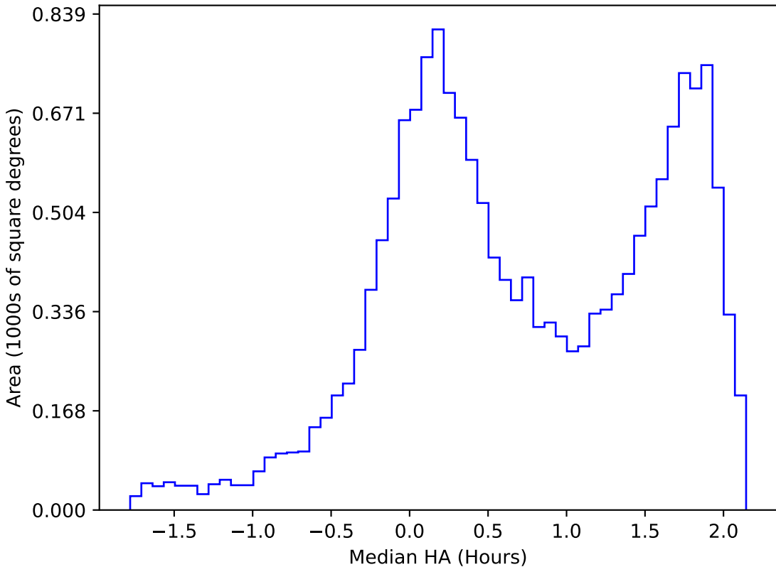
internal_u_expt27_nscale1.1v3.4_10yrs WFD g band: Median HA
