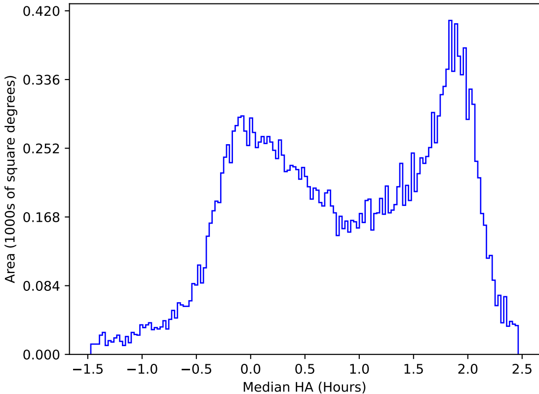
internal_u_expt27_nscale1.1v3.4_10yrs All sky u band: Median HA
