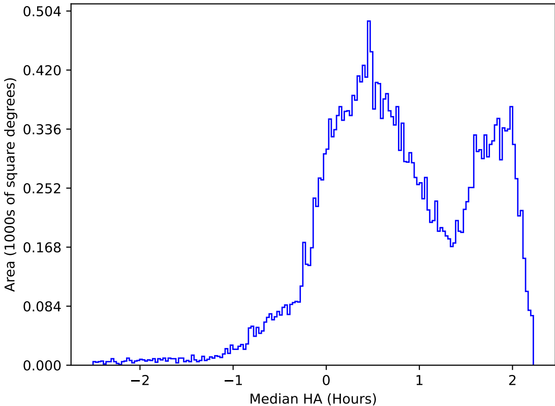
internal_u_expt27_nscale1.1v3.4_10yrs All sky r band: Median HA
