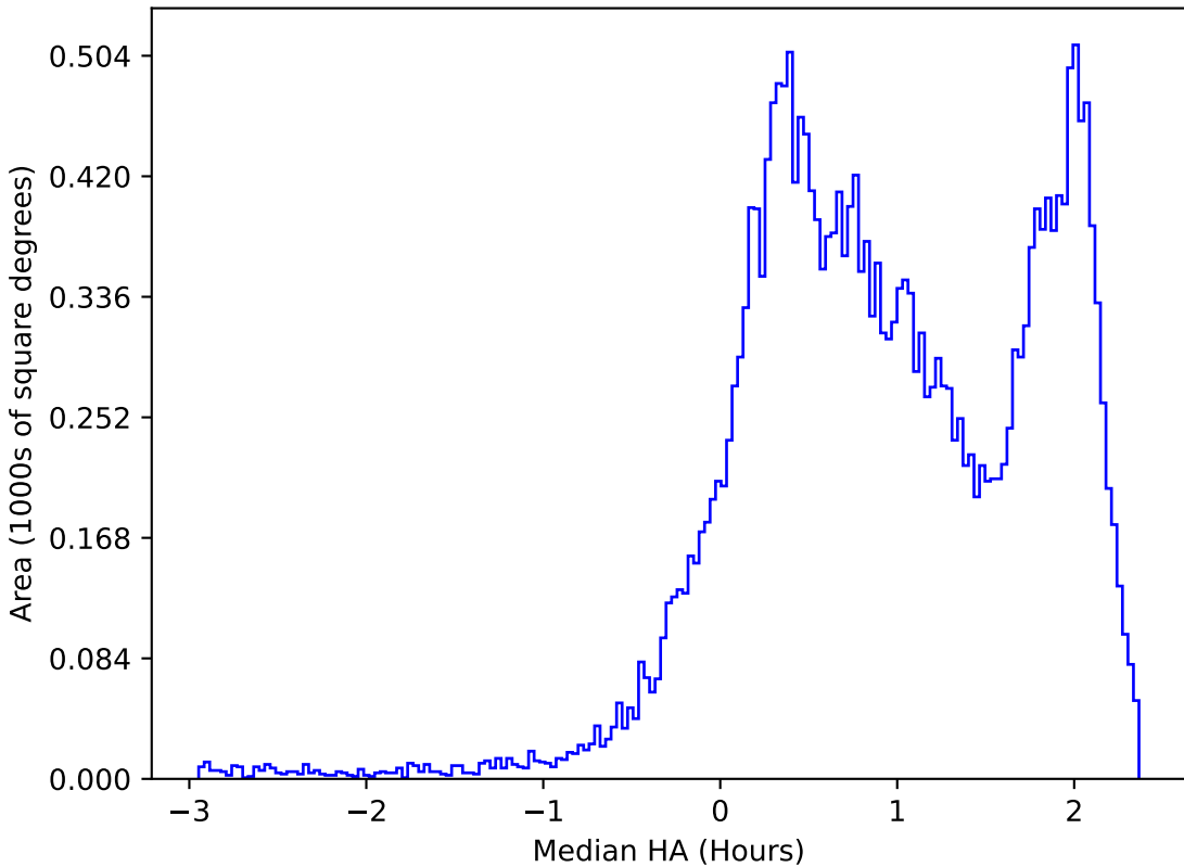
internal_u_expt27_nscale1.1v3.4_10yrs All sky i band: Median HA
