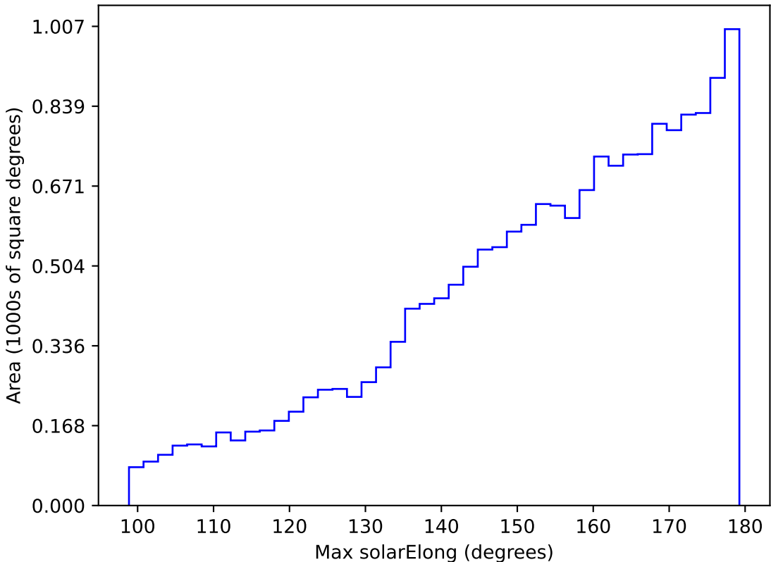
internal_u_expt27_nscale1.1v3.4_10yrs WFD y band: Max solarElong
