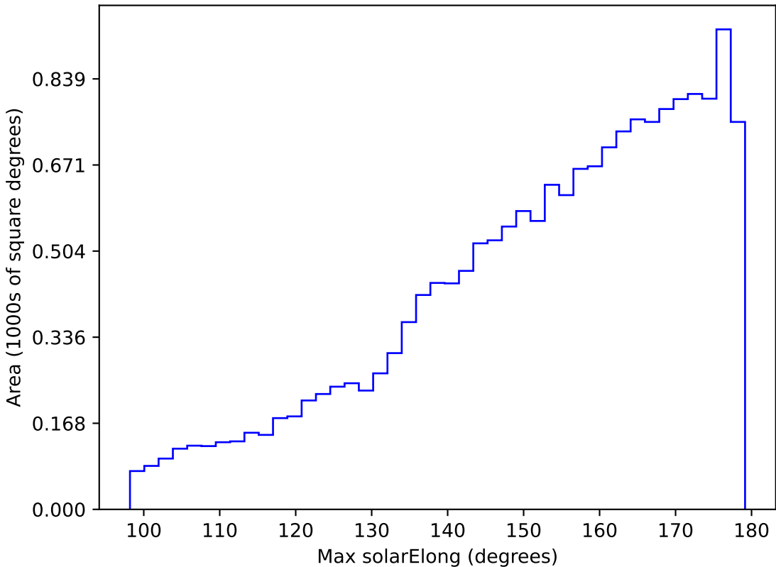
internal_u_expt27_nscale1.1v3.4_10yrs WFD u band: Max solarElong
