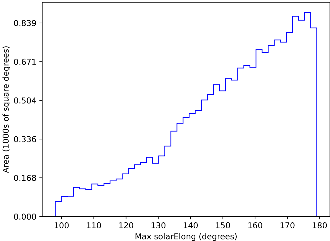
internal_u_expt27_nscale1.1v3.4_10yrs WFD g band: Max solarElong
