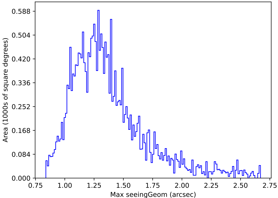
internal_u_expt27_nscale1.1v3.4_10yrs Yr 1 u band: Max seeingGeom
