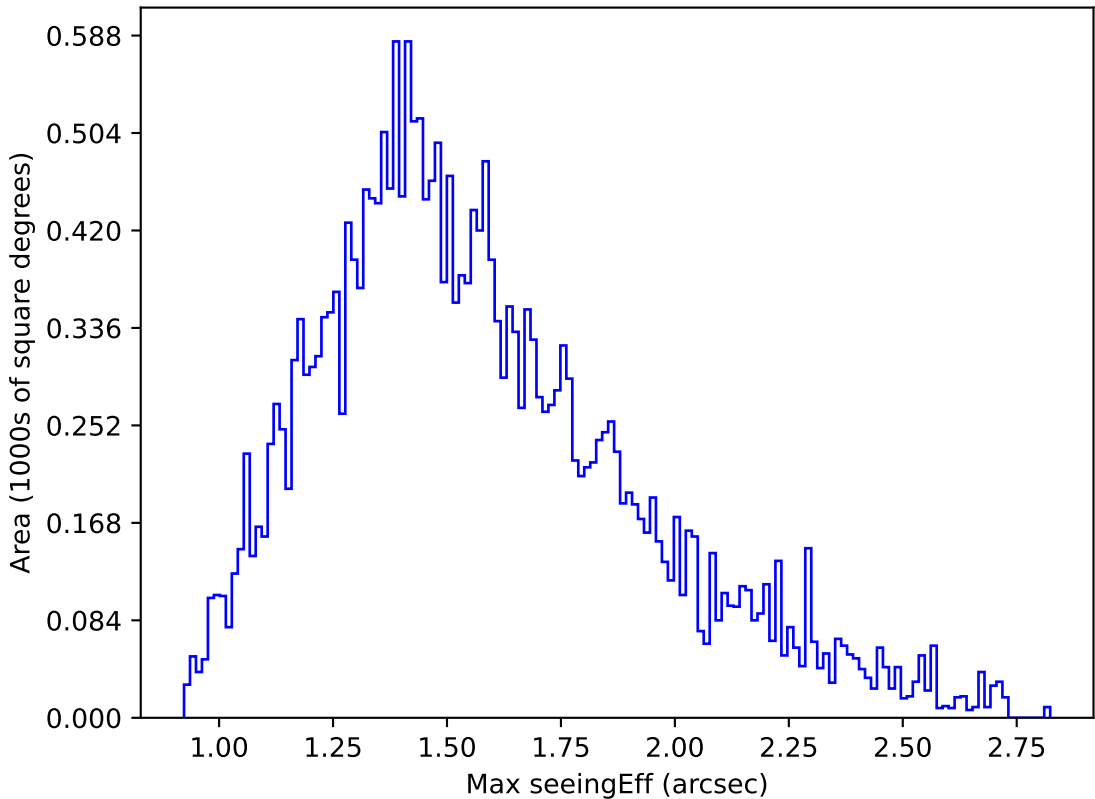
internal_u_expt27_nscale1.1v3.4_10yrs Yr 1 r band: Max seeingEff
