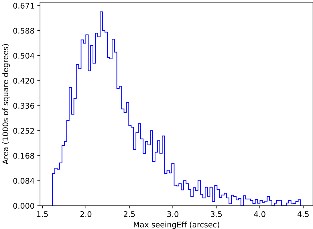
internal_u_expt27_nscale1.1v3.4_10yrs WFD y band: Max seeingEff
