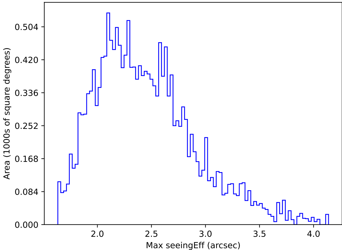
internal_u_expt27_nscale1.1v3.4_10yrs WFD g band: Max seeingEff
