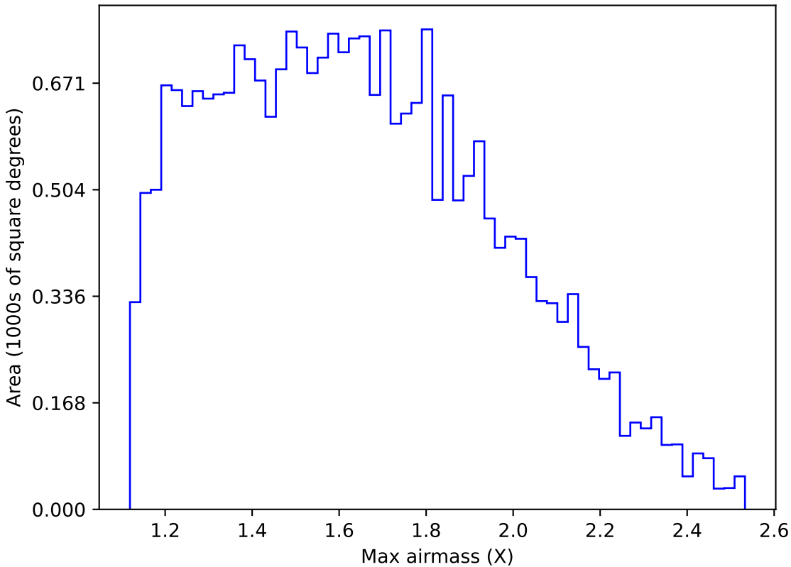
internal_u_expt27_nscale1.1v3.4_10yrs Yr 1 g band: Max airmass
