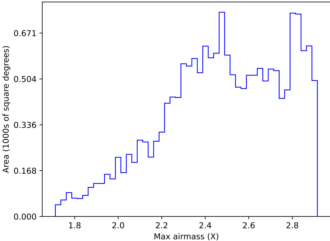
internal_u_expt27_nscale1.1v3.4_10yrs WFD z band: Max airmass
