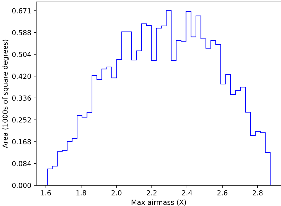
internal_u_expt27_nscale1.1v3.4_10yrs WFD y band: Max airmass
