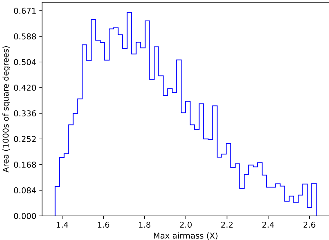
internal_u_expt27_nscale1.1v3.4_10yrs WFD u band: Max airmass
