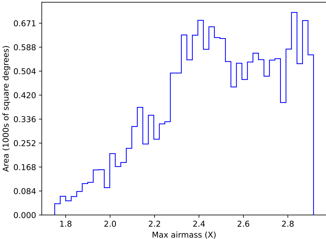
internal_u_expt27_nscale1.1v3.4_10yrs WFD i band: Max airmass
