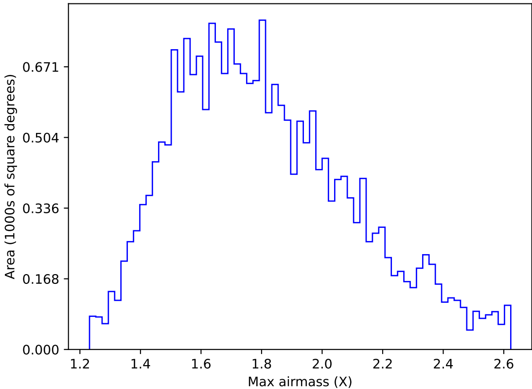
internal_u_expt27_nscale1.1v3.4_10yrs All sky u band: Max airmass
