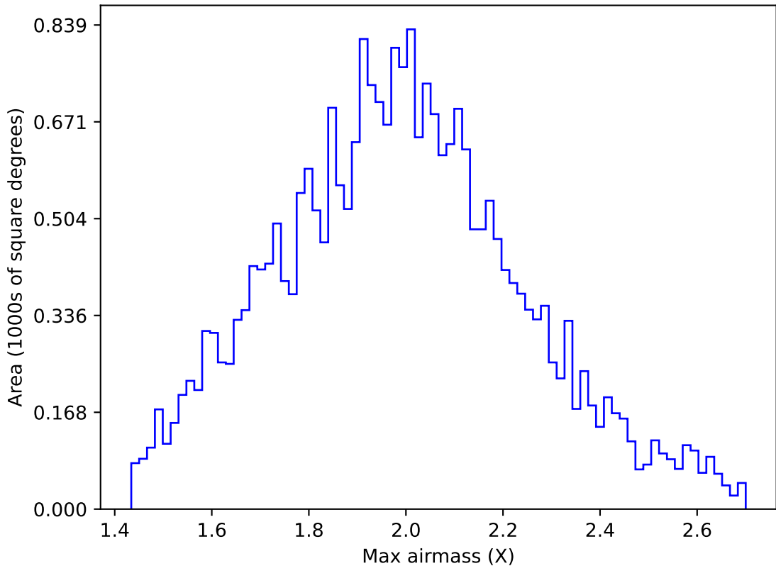
internal_u_expt27_nscale1.1v3.4_10yrs All sky g band: Max airmass
