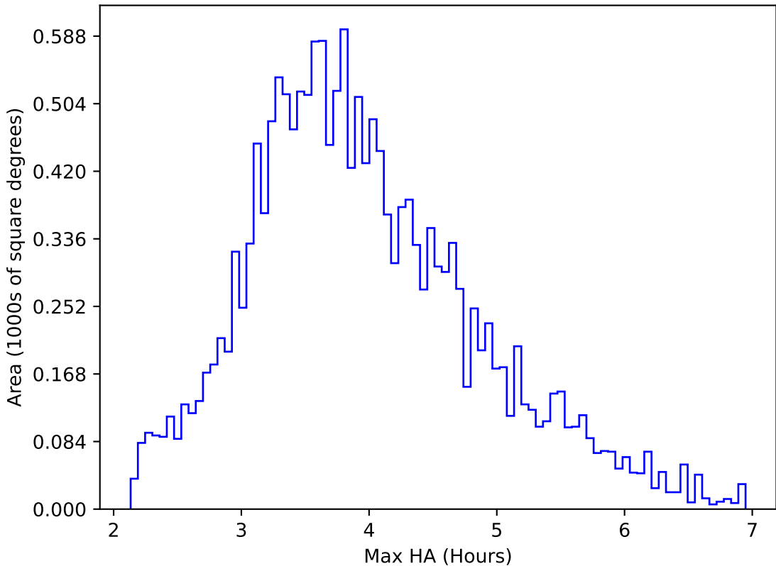
internal_u_expt27_nscale1.1v3.4_10yrs WFD u band: Max HA
