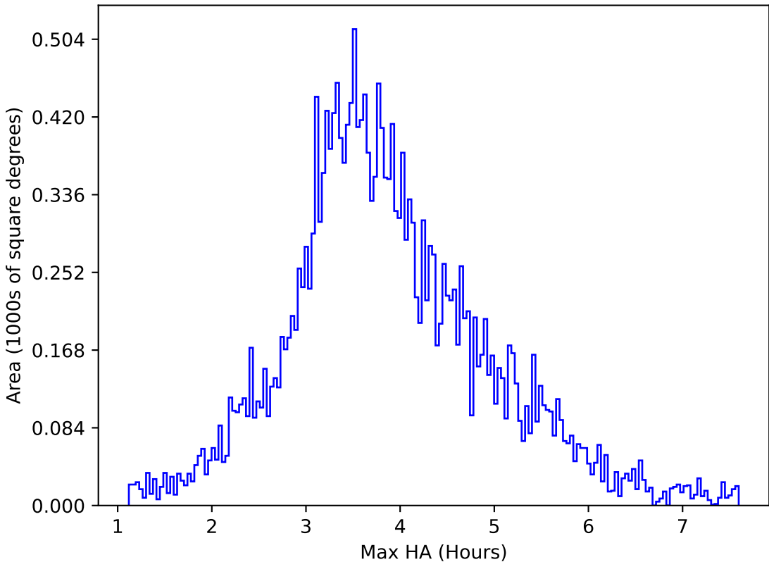
internal_u_expt27_nscale1.1v3.4_10yrs All sky u band: Max HA
