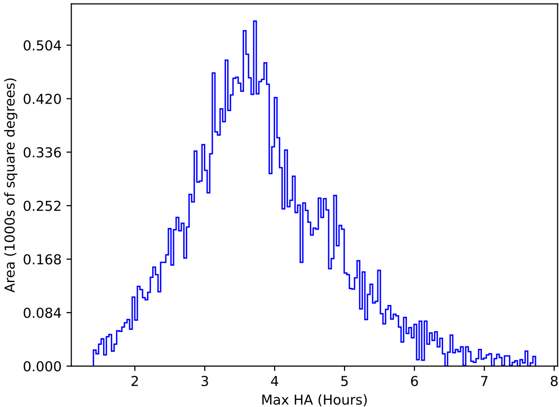
internal_u_expt27_nscale1.1v3.4_10yrs All sky g band: Max HA
