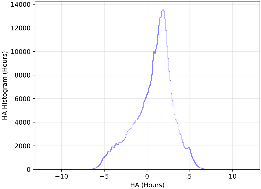
internal_u_expt27_nscale1.1v3.4_10yrs WFD z band: HA Histogram
