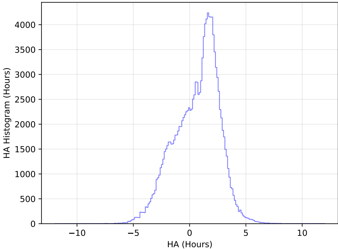
internal_u_expt27_nscale1.1v3.4_10yrs WFD u band: HA Histogram
