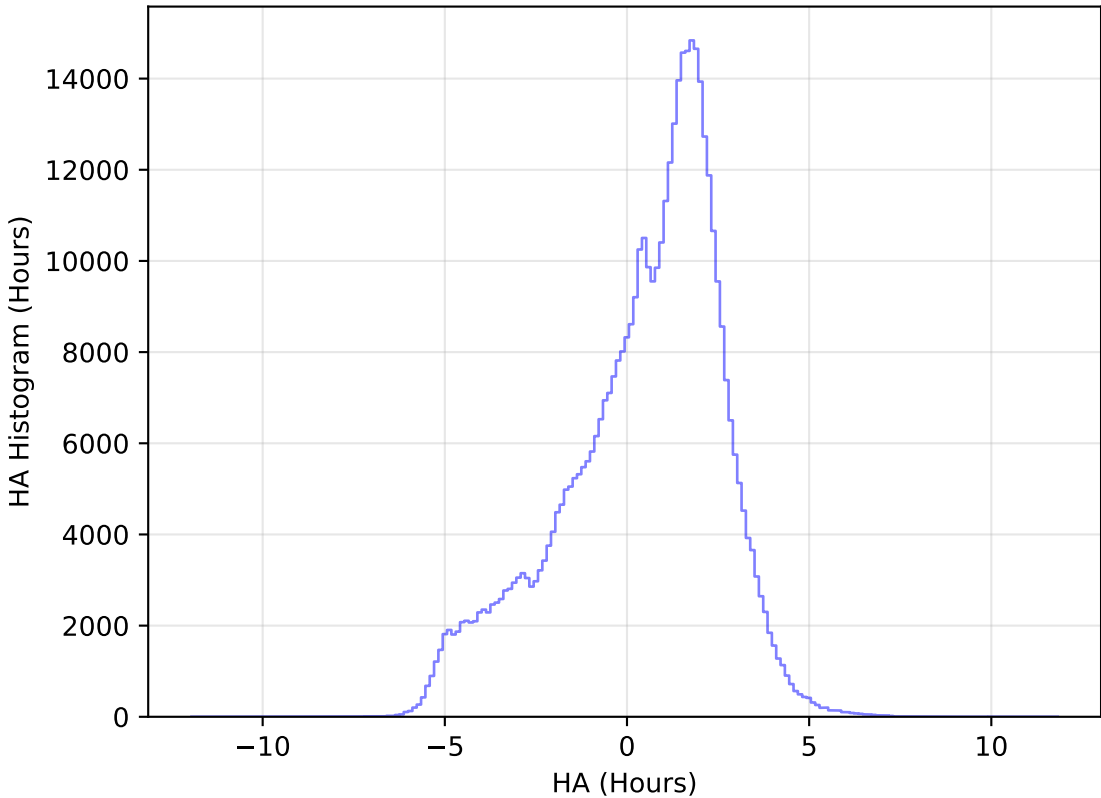
internal_u_expt27_nscale1.1v3.4_10yrs WFD r band: HA Histogram
