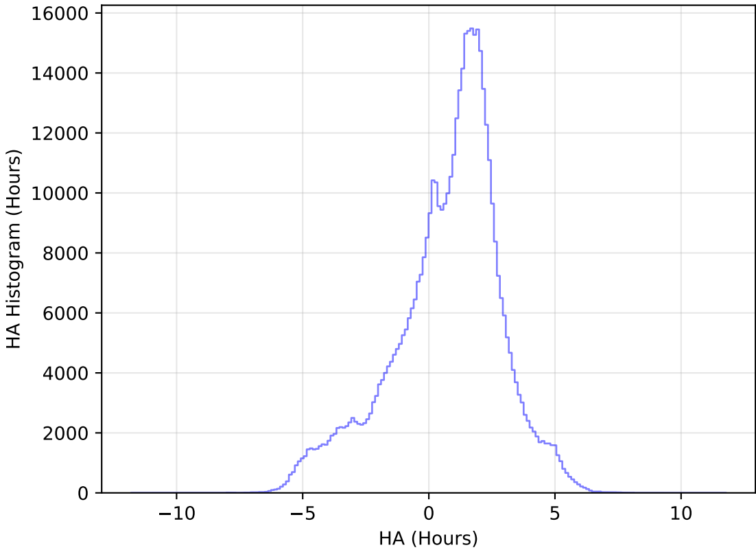
internal_u_expt27_nscale1.1v3.4_10yrs WFD i band: HA Histogram
