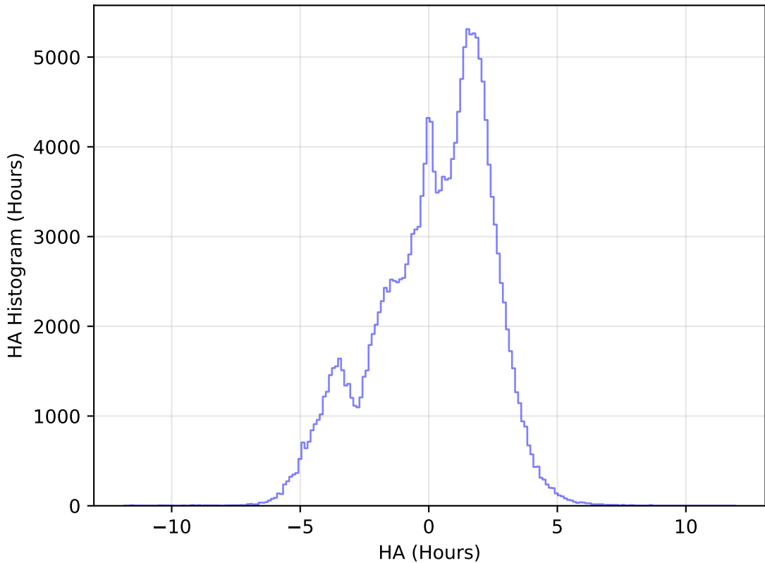
internal_u_expt27_nscale1.1v3.4_10yrs WFD g band: HA Histogram
