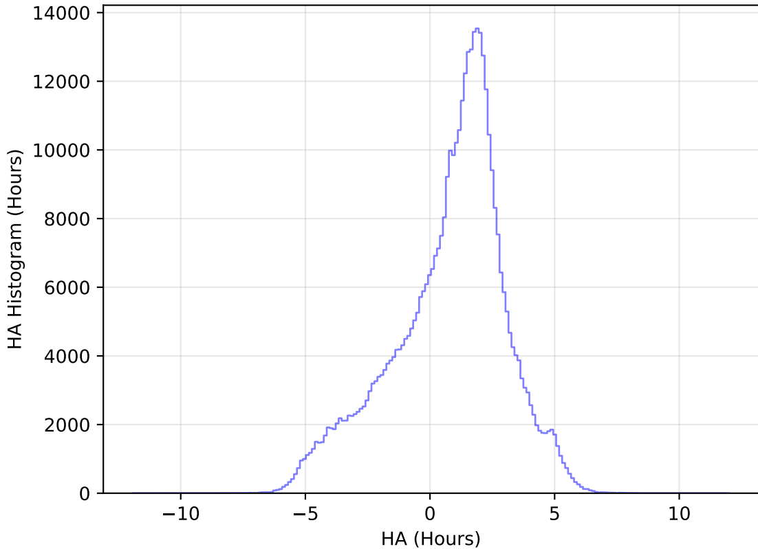
internal_u_expt27_nscale1.1v3.4_10yrs All sky z band: HA Histogram
