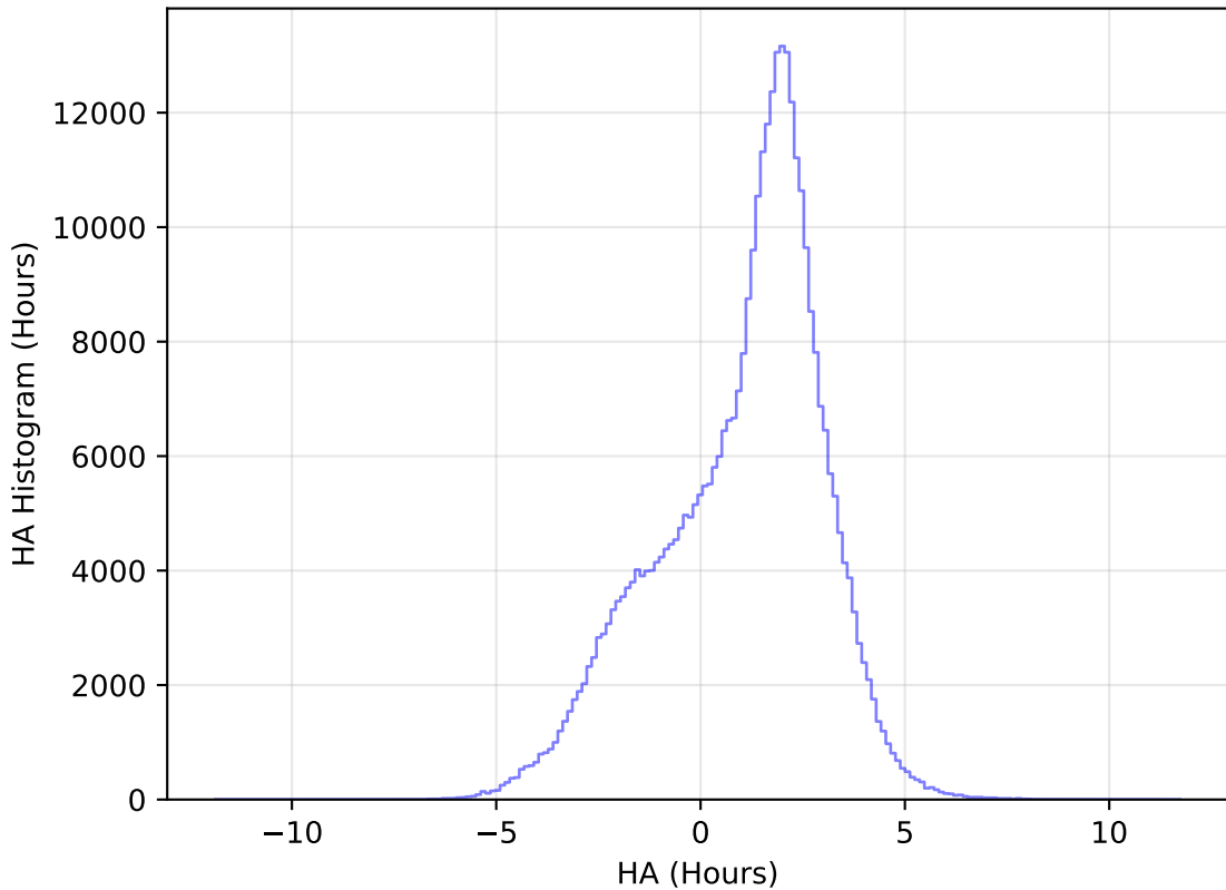
internal_u_expt27_nscale1.1v3.4_10yrs All sky y band: HA Histogram
