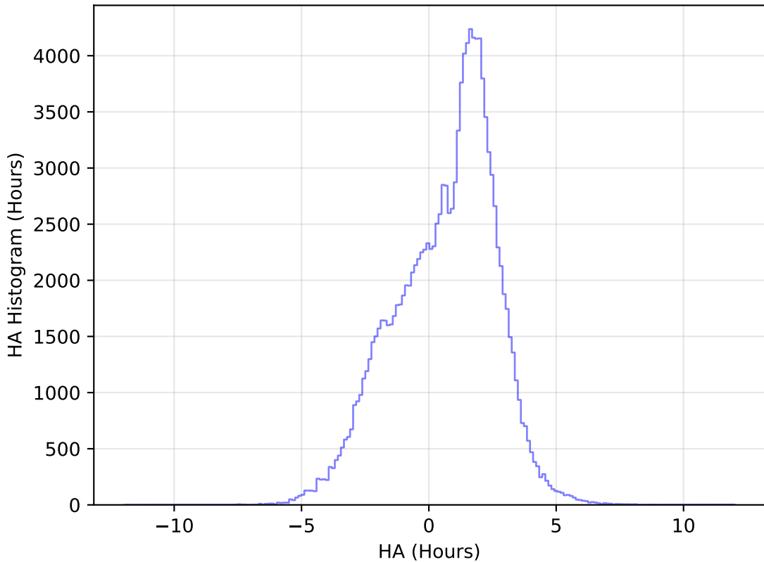
internal_u_expt27_nscale1.1v3.4_10yrs All sky u band: HA Histogram
