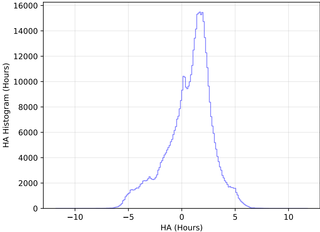
internal_u_expt27_nscale1.1v3.4_10yrs All sky i band: HA Histogram
