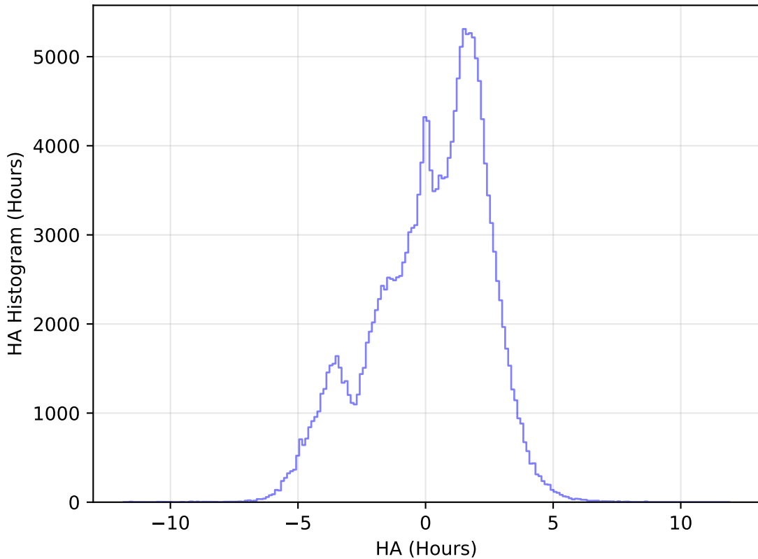
internal_u_expt27_nscale1.1v3.4_10yrs All sky g band: HA Histogram
