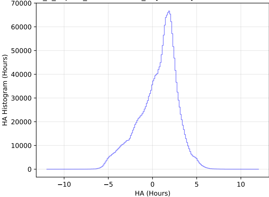
internal_u_expt27_nscale1.1v3.4_10yrs All sky all bands: HA Histogram
