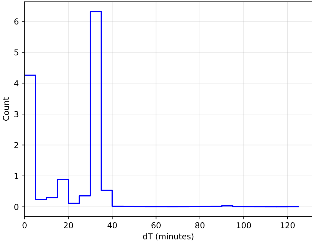
internal_u_expt27_nscale1.1v3.4_10yrs All sky: DeltaT Histogram 1e6
