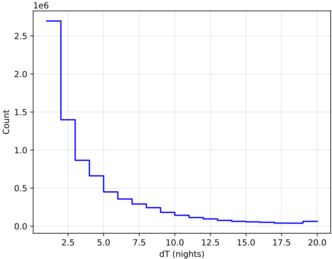
internal_u_expt27_nscale1.1v3.4_10yrs WFD all bands: DeltaNight Histogram
