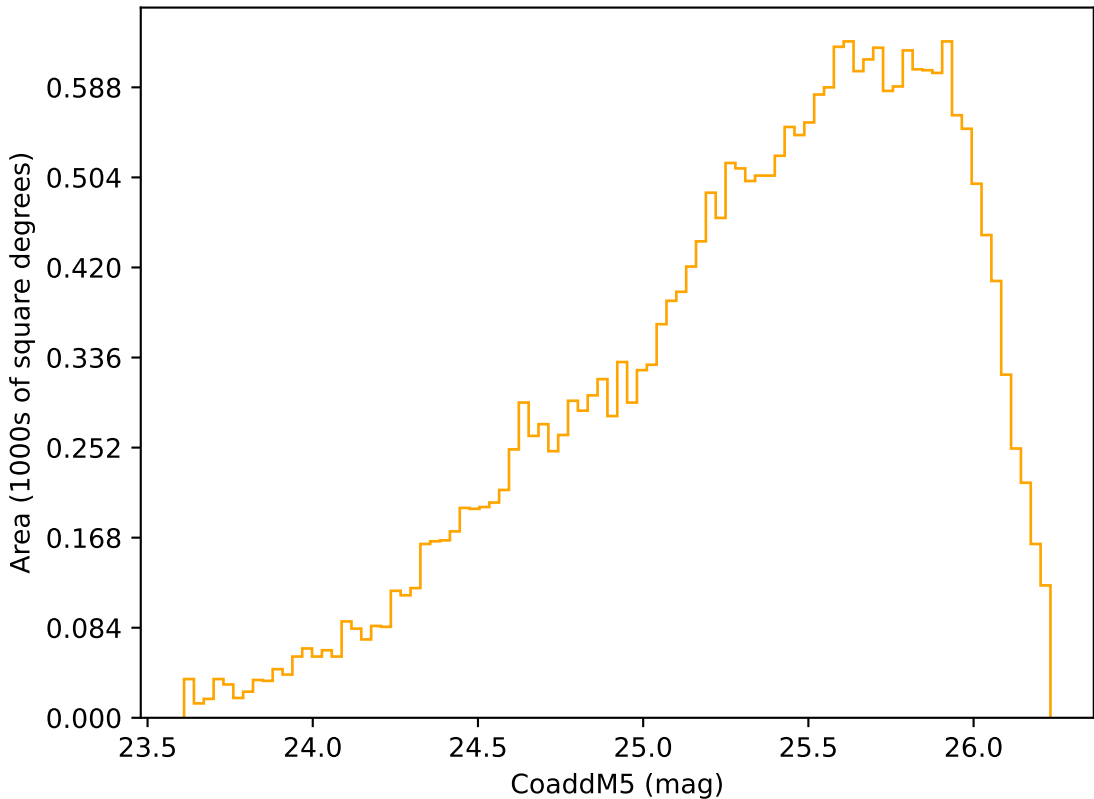
internal_u_expt27_nscale1.1v3.4_10yrs Yr 3-4 r band: CoaddM5
