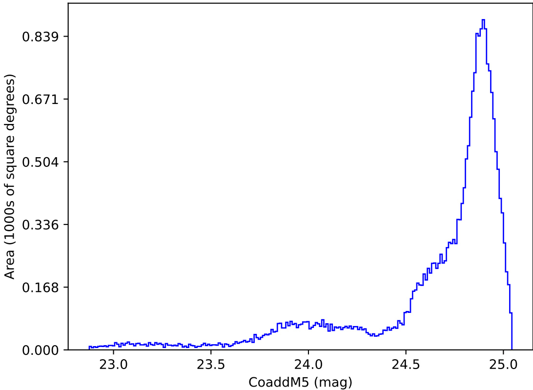
internal_u_expt27_nscale1.1v3.4_10yrs All sky y band: CoaddM5
