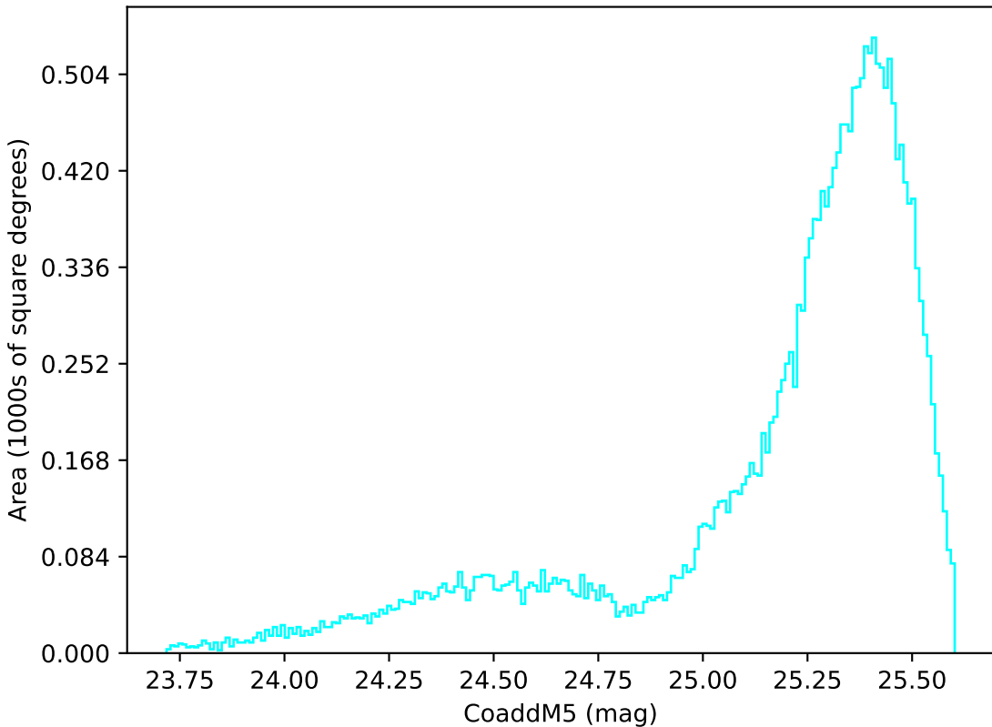
internal_u_expt27_nscale1.1v3.4_10yrs All sky u band: CoaddM5
