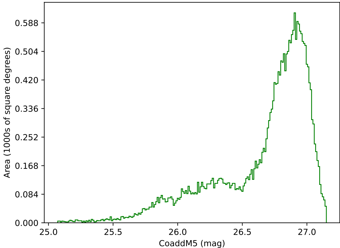
internal_u_expt27_nscale1.1v3.4_10yrs All sky g band: CoaddM5
