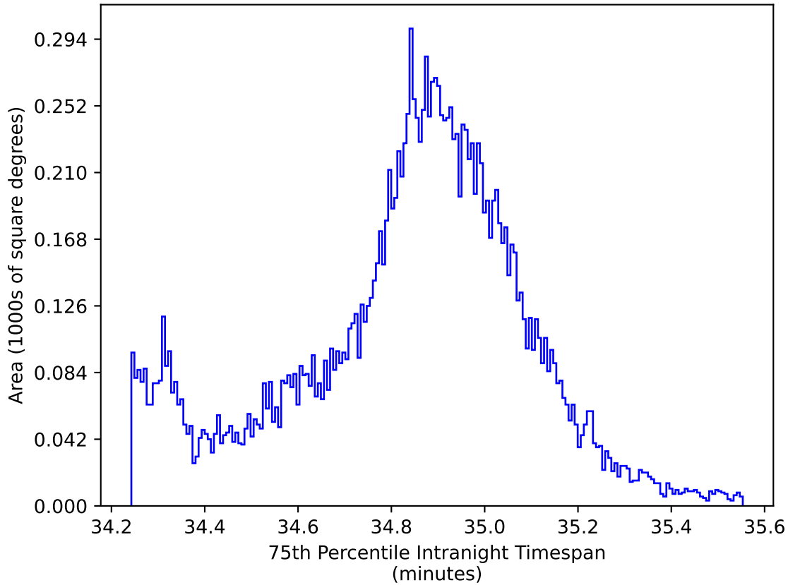
internal_u_expt27_nscale1.1v3.4_10yrs WFD all bands: 75th Percentile Intranight Timespan
