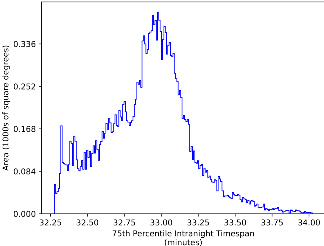
internal_u_expt27_nscale1.1v3.4_10yrs All sky y band: 75th Percentile Intranight Timespan
