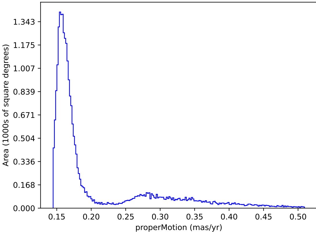
internal_u_expt27_nscale1.1v3.4_10yrs : properMotion
