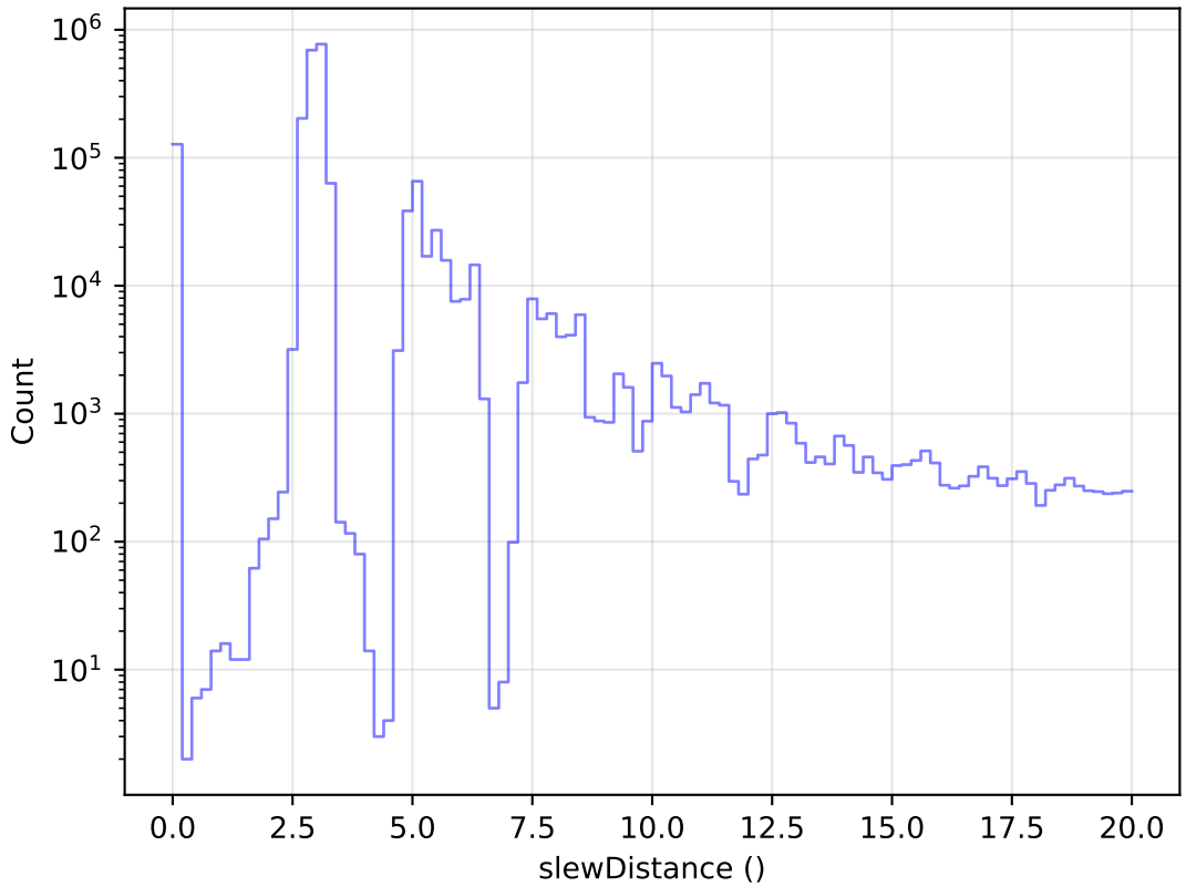
internal_u_expt27_nscale1.1v3.4_10yrs All visits: Zoom Slew Distance Histogram
