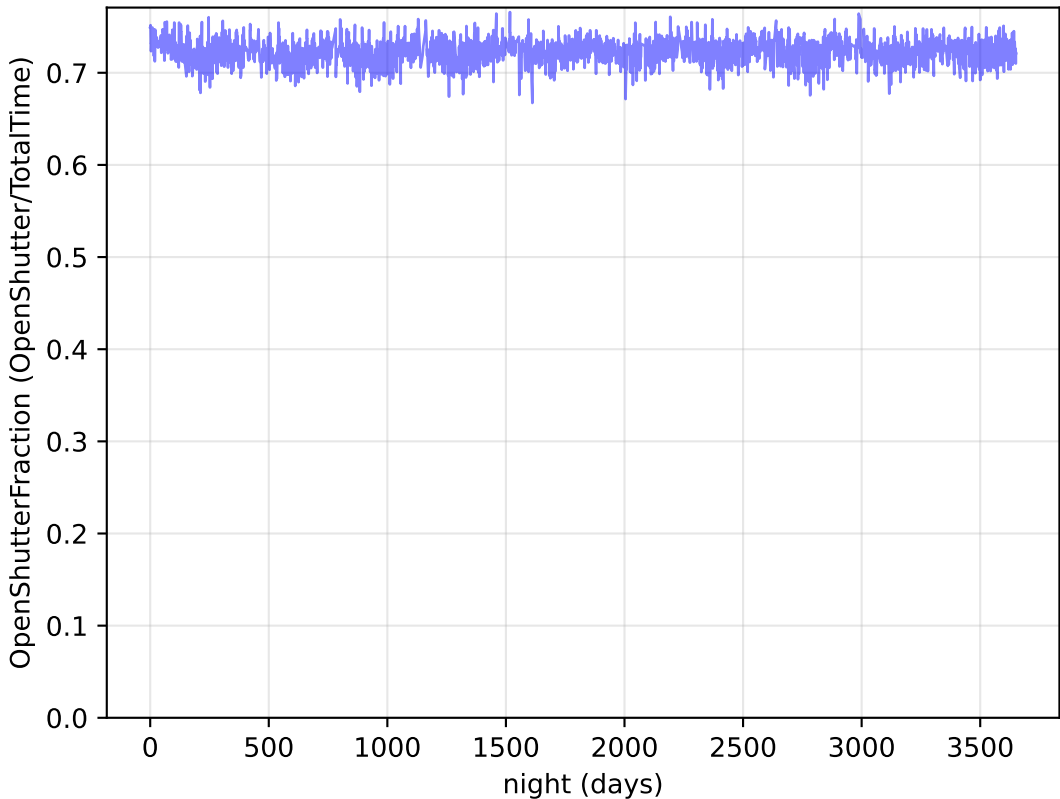
internal_u_expt27_nscale1.1v3.4_10yrs : OpenShutterFraction
