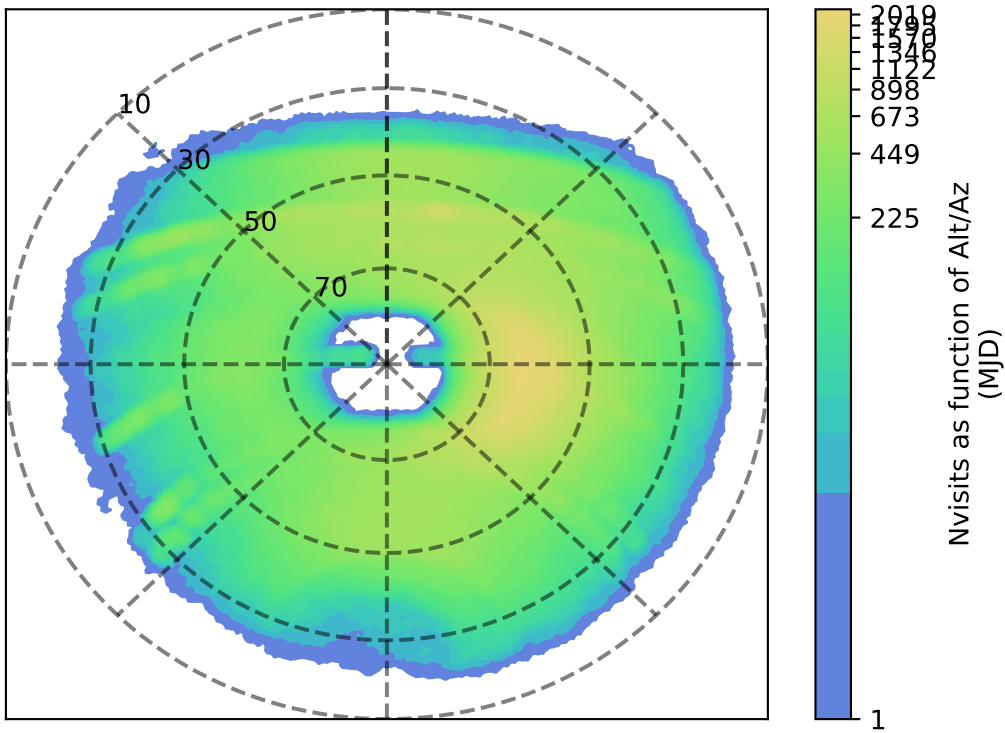
internal_u_expt27_nscale1.1v3.4_10yrs y: Nvisits as function of Alt/Az
