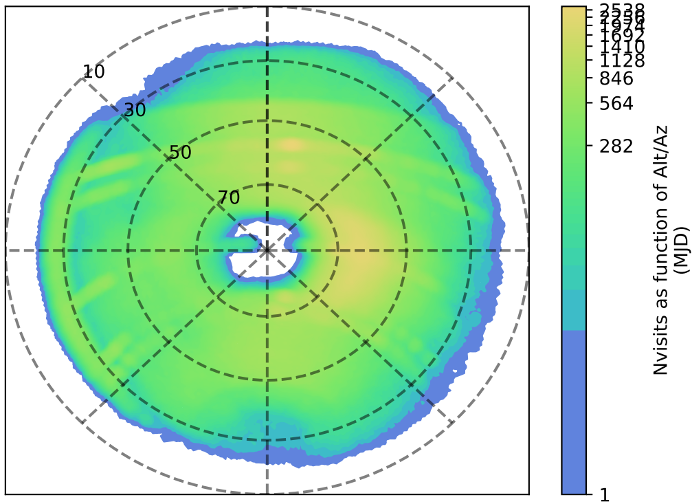
internal_u_expt27_nscale1.1v3.4_10yrs r: Nvisits as function of Alt/Az
