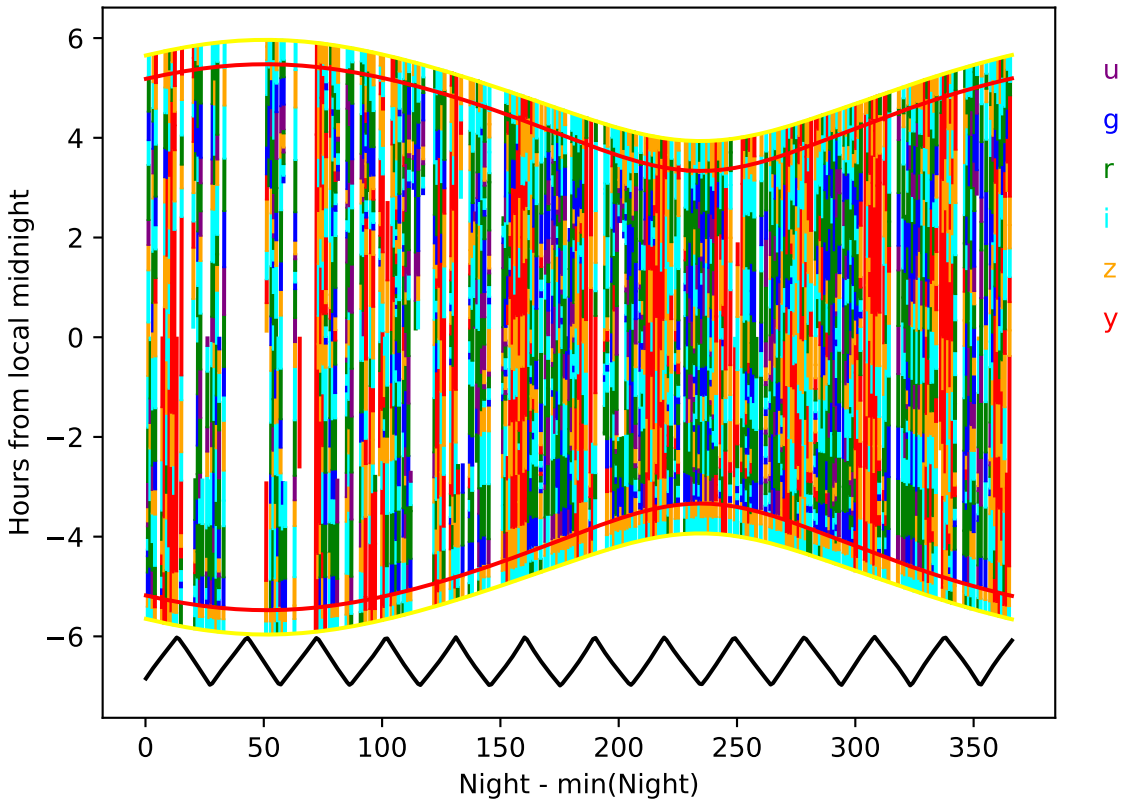
internal_u_expt27_nscale1.1v3.4_10yrs year 8-9: Hourglass
