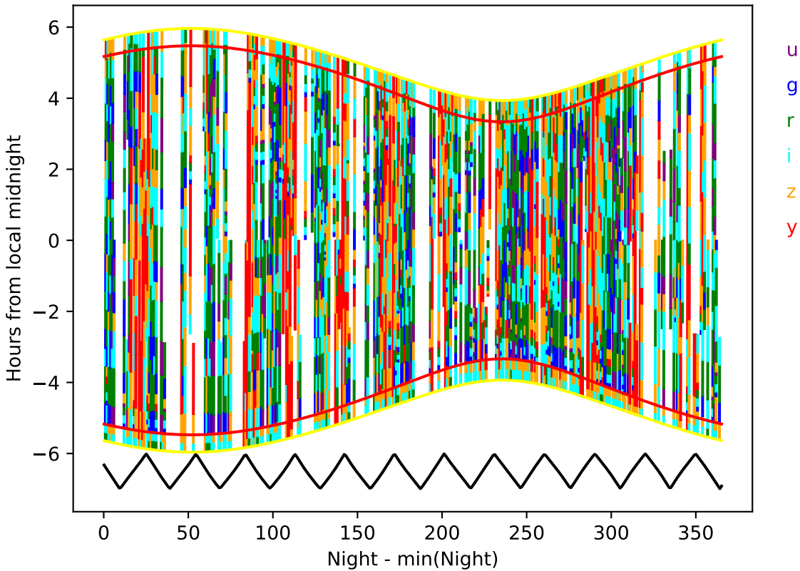
internal_u_expt27_nscale1.1v3.4_10yrs year 7-8: Hourglass
