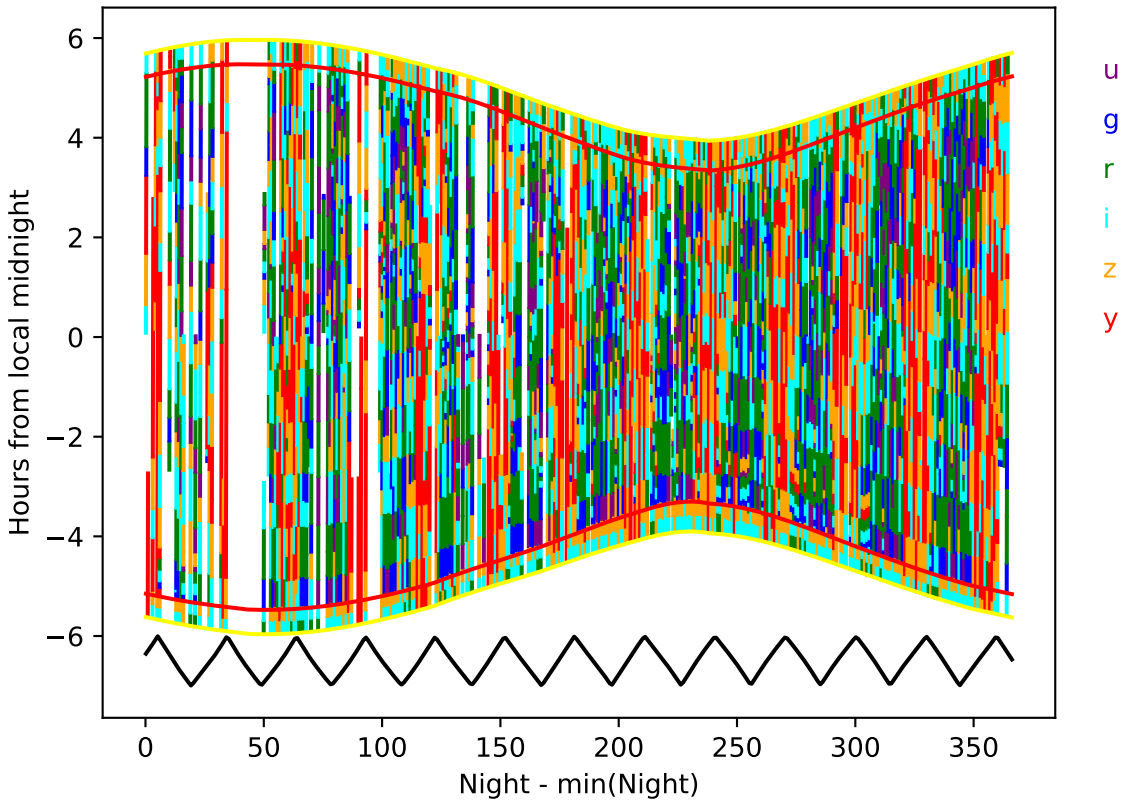
internal_u_expt27_nscale1.1v3.4_10yrs year 6-7: Hourglass
