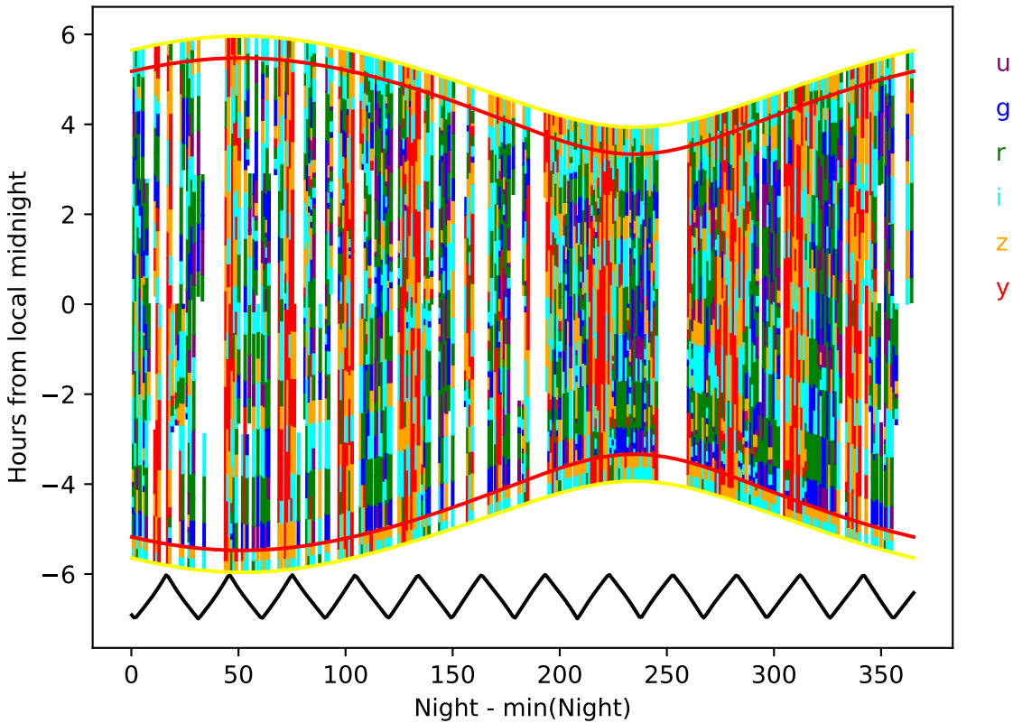
internal_u_expt27_nscale1.1v3.4_10yrs year 5-6: Hourglass
